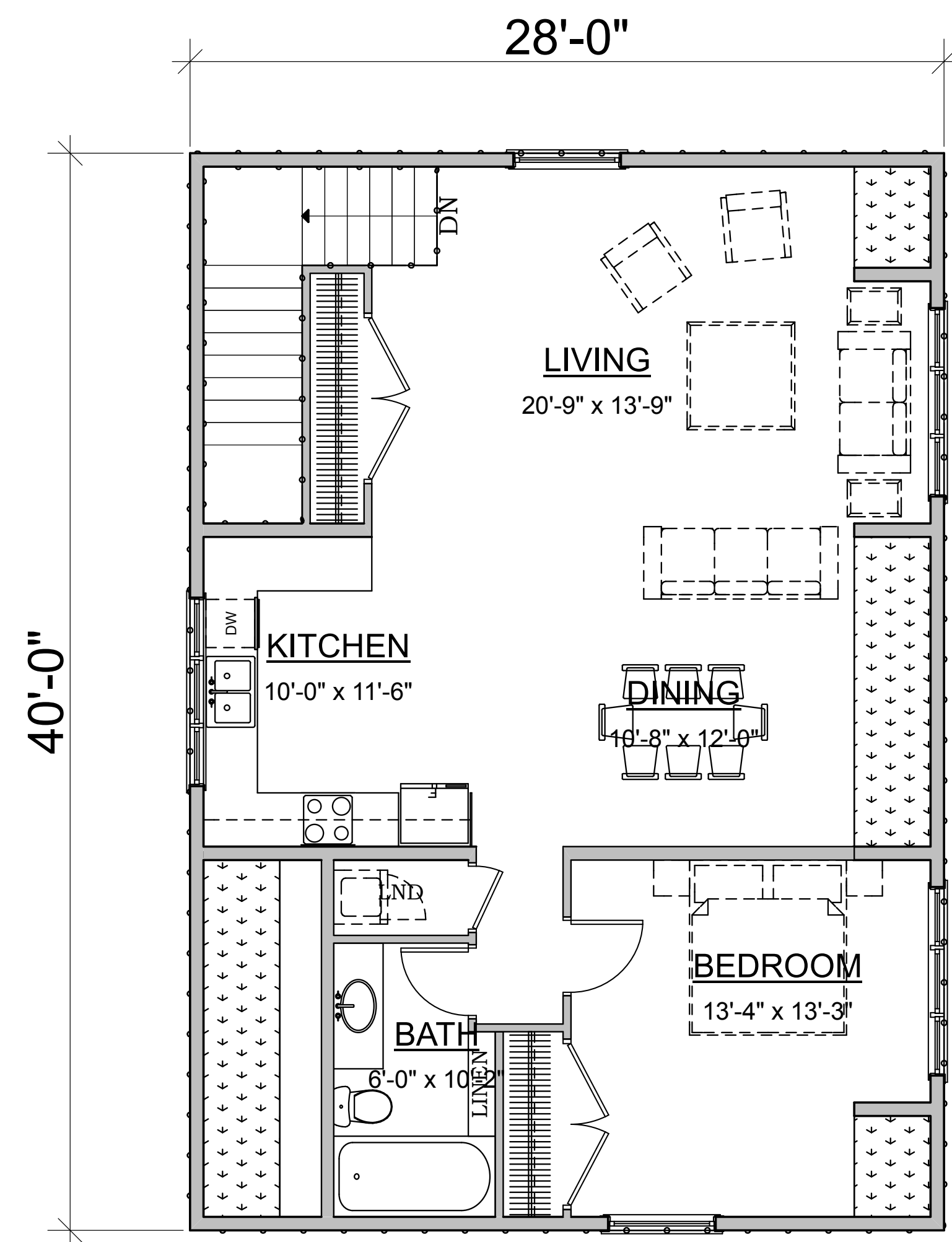
GUEST SUITE AREA: 929 sq ft
