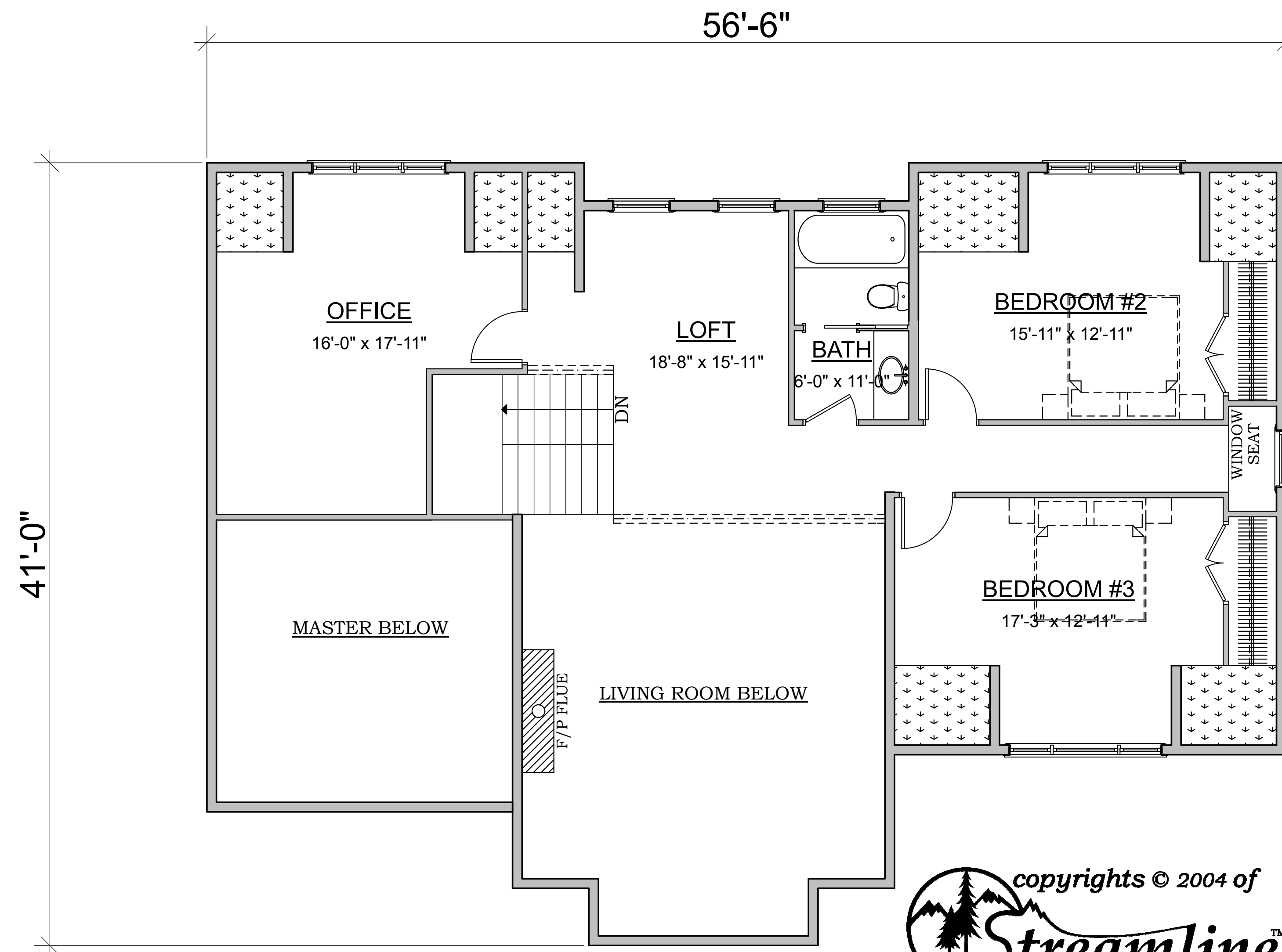
SECOND FLOOR PLAN AREA: 1,063 sq ft
