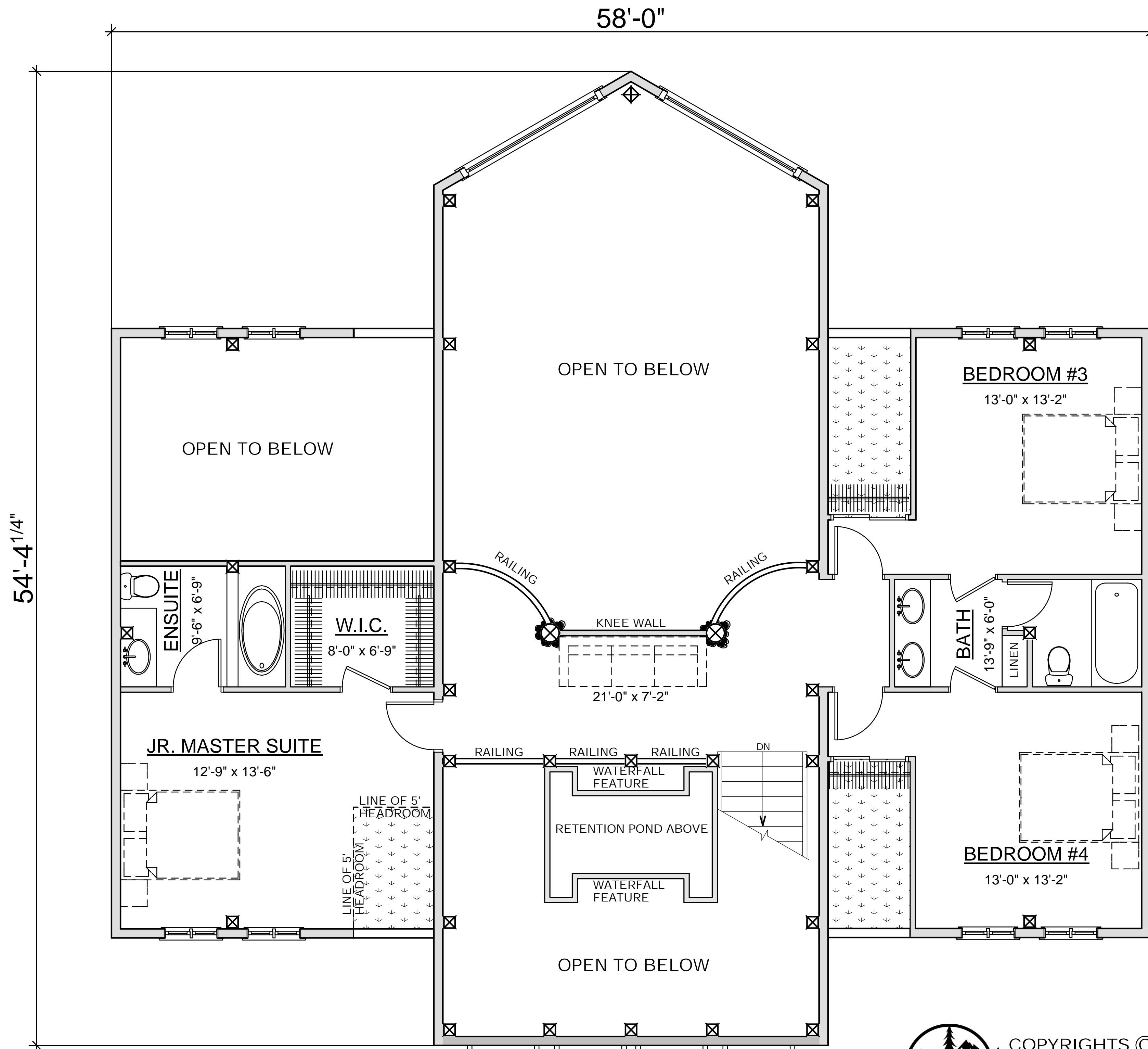
SECOND FLOOR PLAN AREA: 1,366 SQ. FT. BONUS ROOM AREA 733 SQ.FT.
