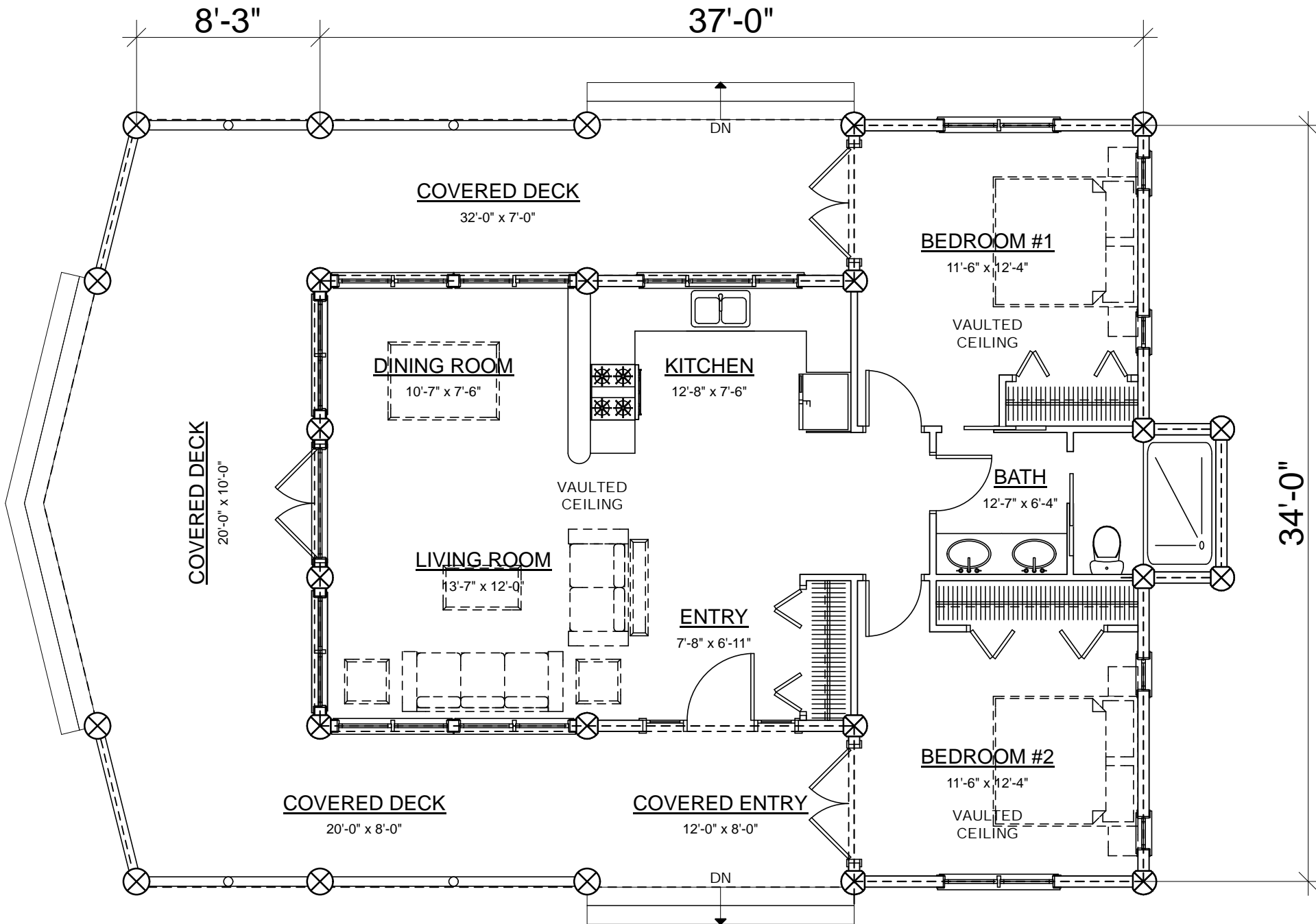
FIRST FLOOR PLAN AREA: 980 SQ. FT.
