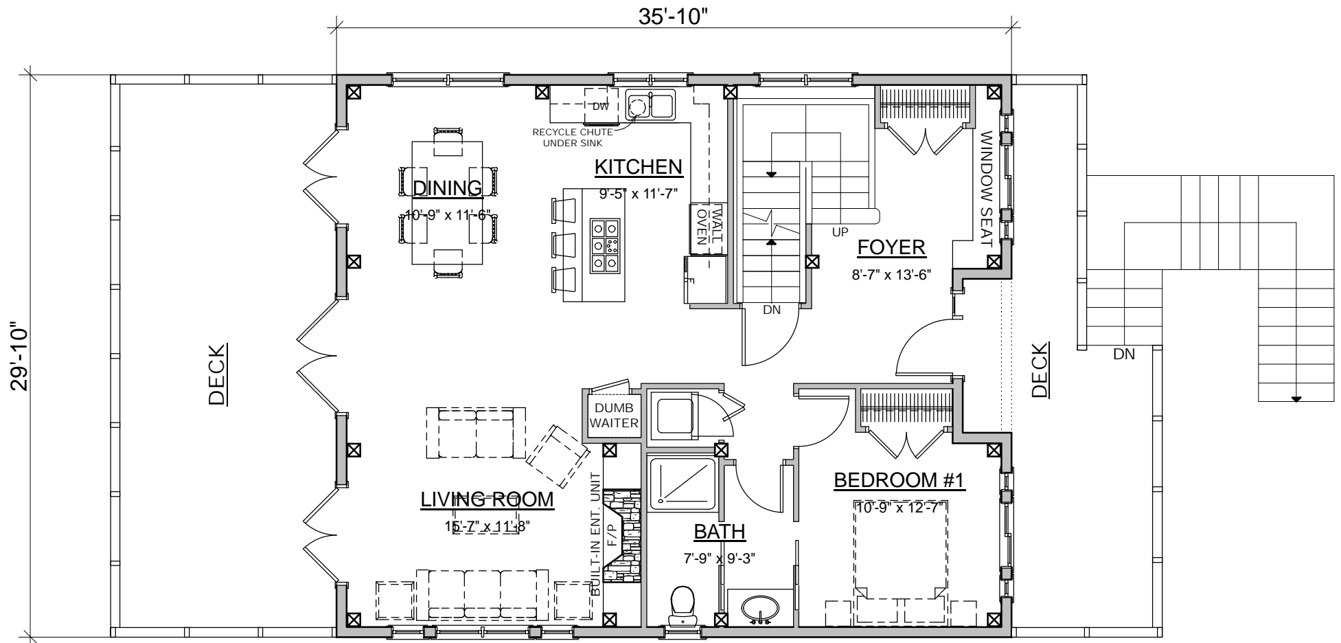
FIRST FLOOR PLAN AREA: 1049 SQ.FT.
