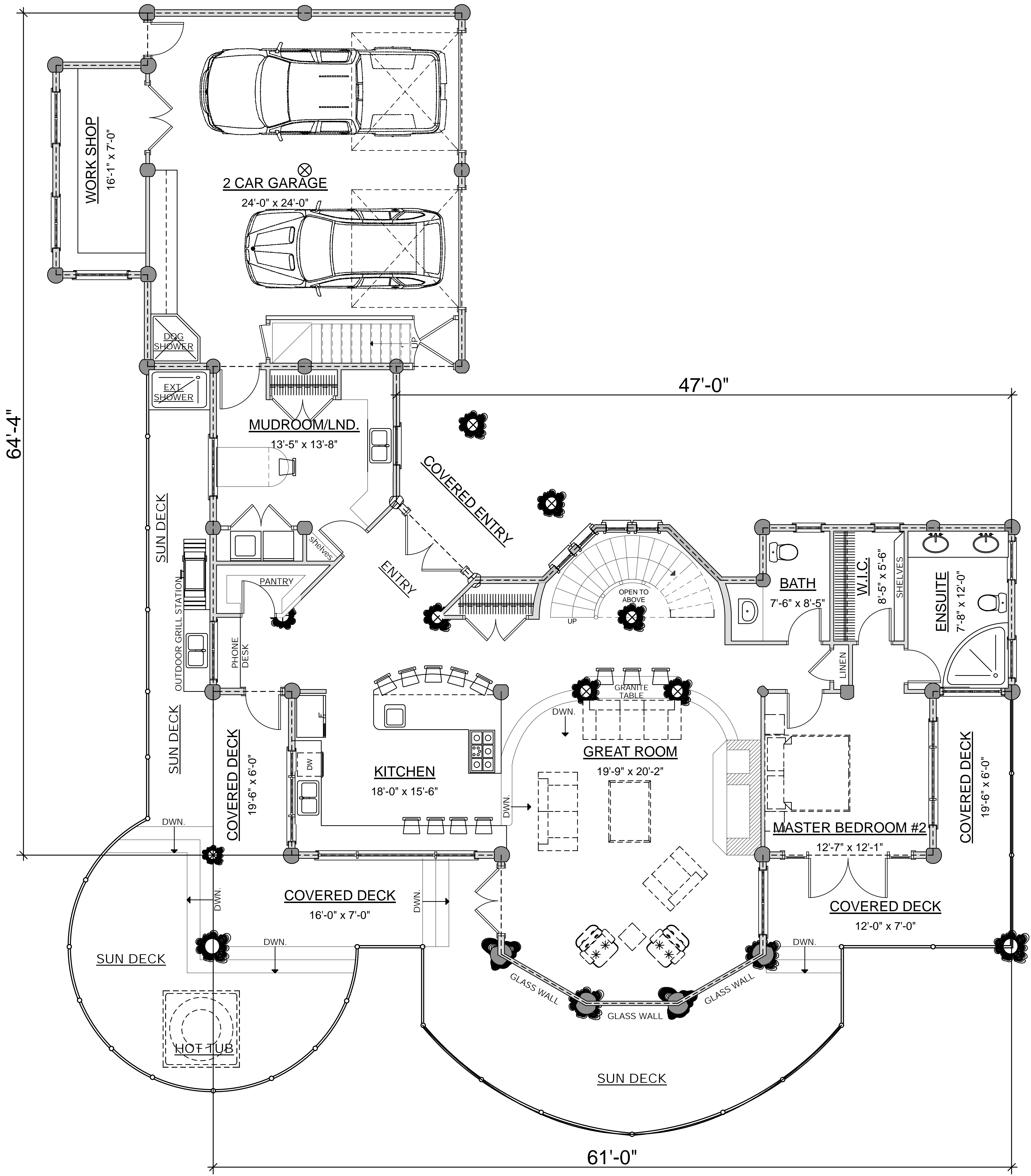
FIRST FLOOR PLAN AREA: 1,743 SQ.FT.
