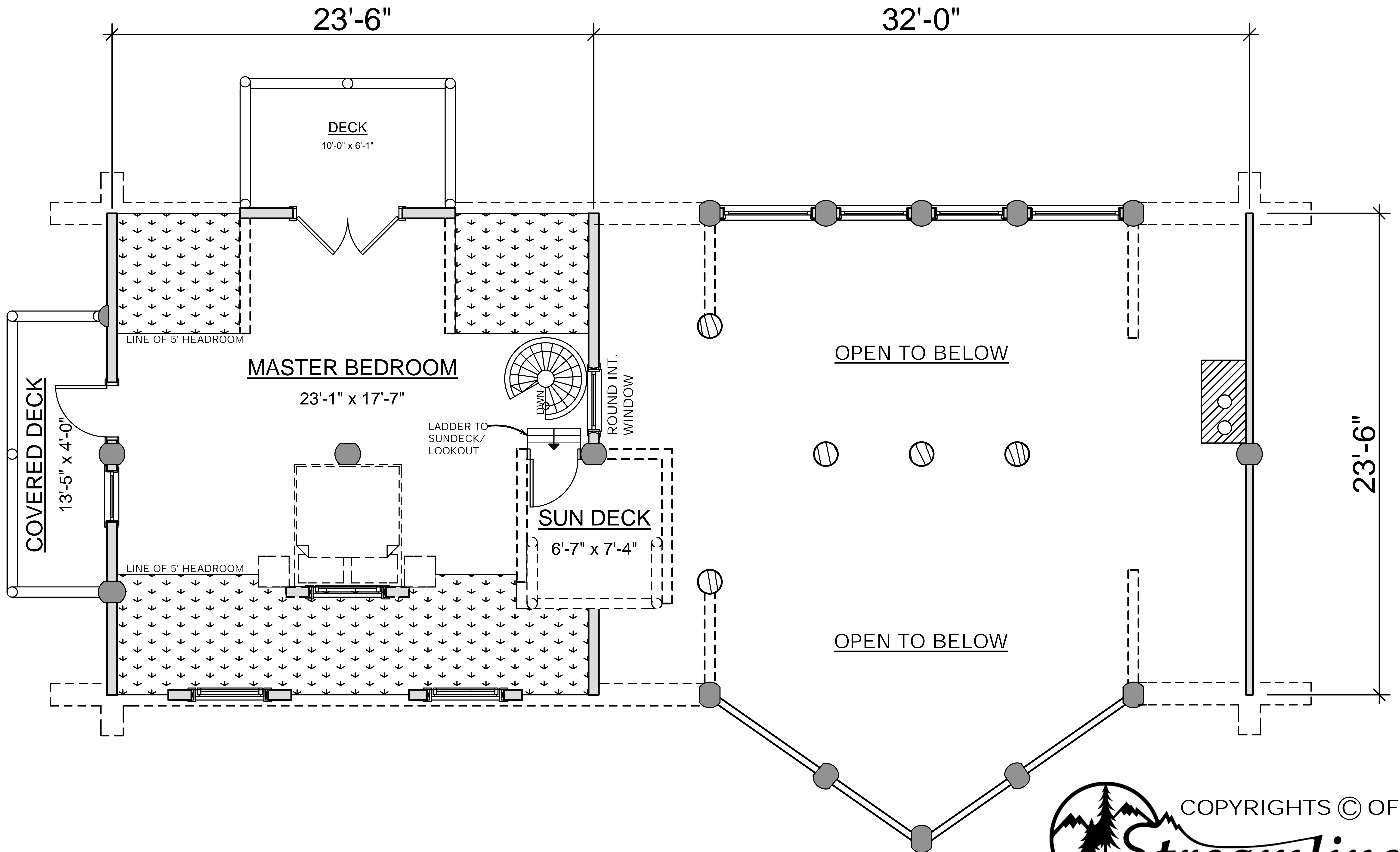
SECOND FLOOR PLAN AREA: 345 SQ. FT.
