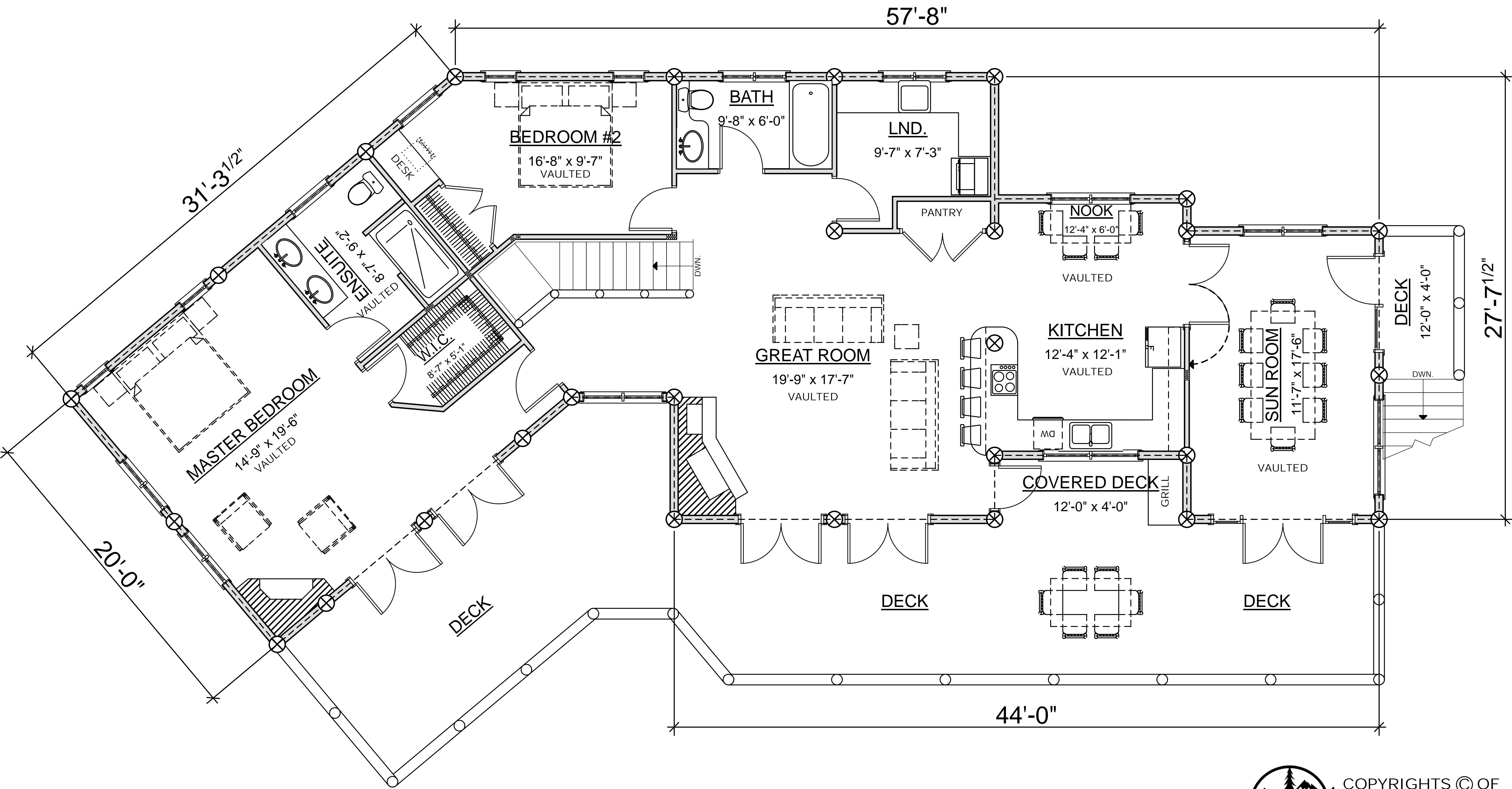
MAIN FLOOR PLAN AREA: 1,770 SQ.FT.
