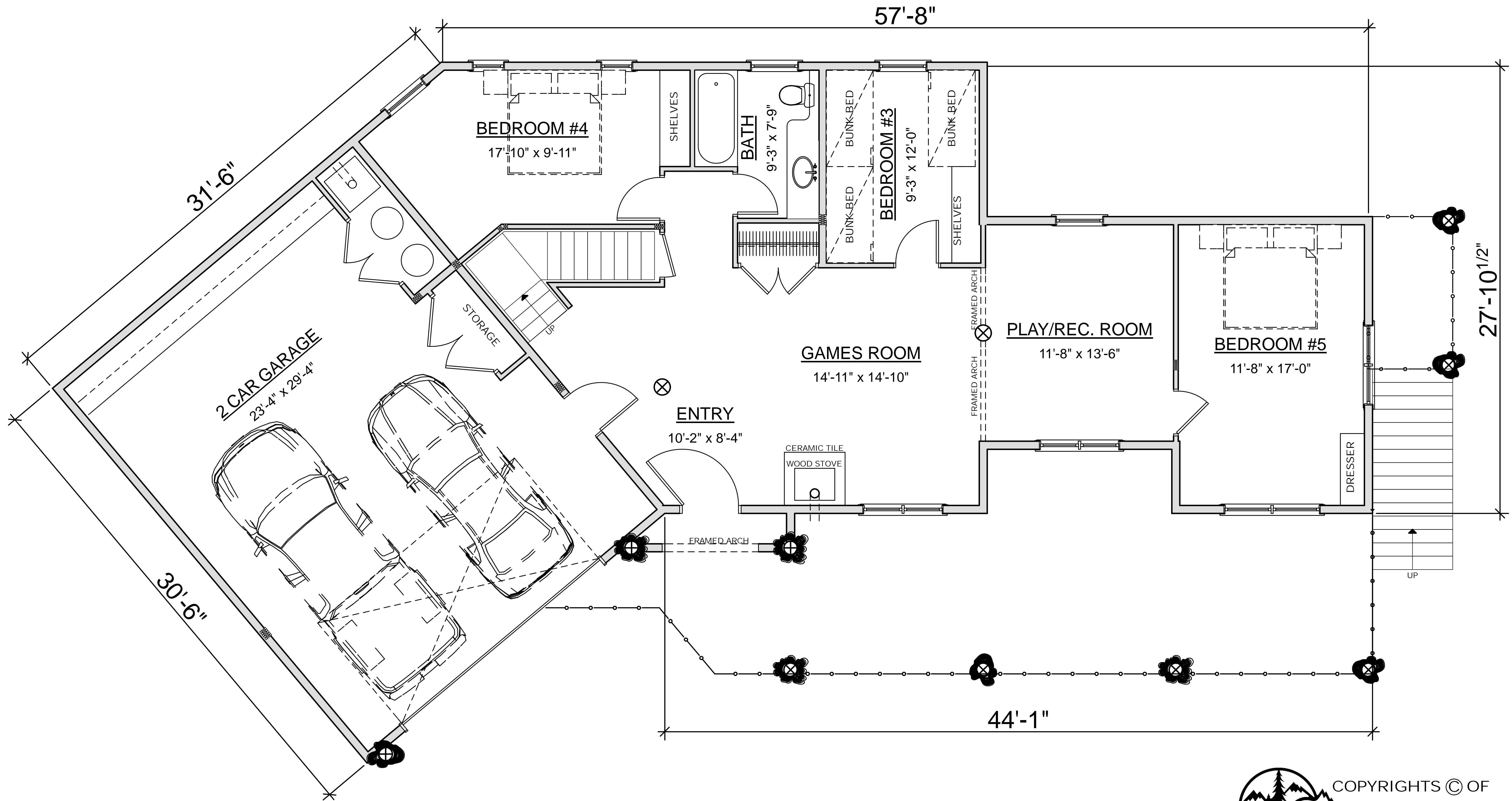
FIRST FLOOR PLAN AREA: 1, 270 SQ. FT. GARAGE AREA: 720 SQ. FT.
