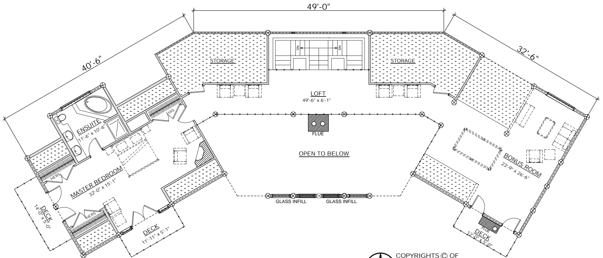
SECOND FLOOR PLAN AREA: 1,802 SQ. FT.
