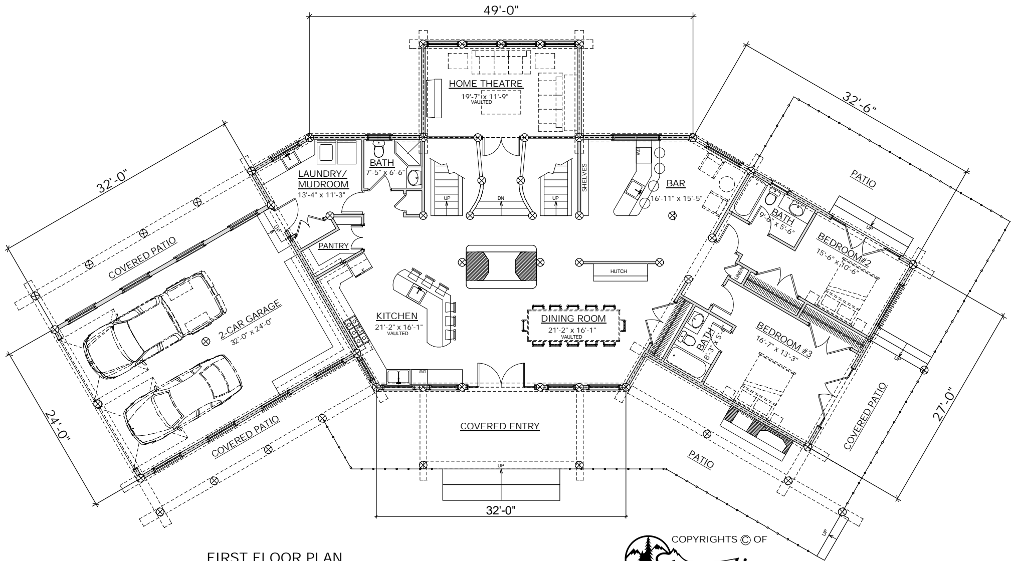
FIRST FLOOR PLAN AREA: 2,510 SQ.FT.
