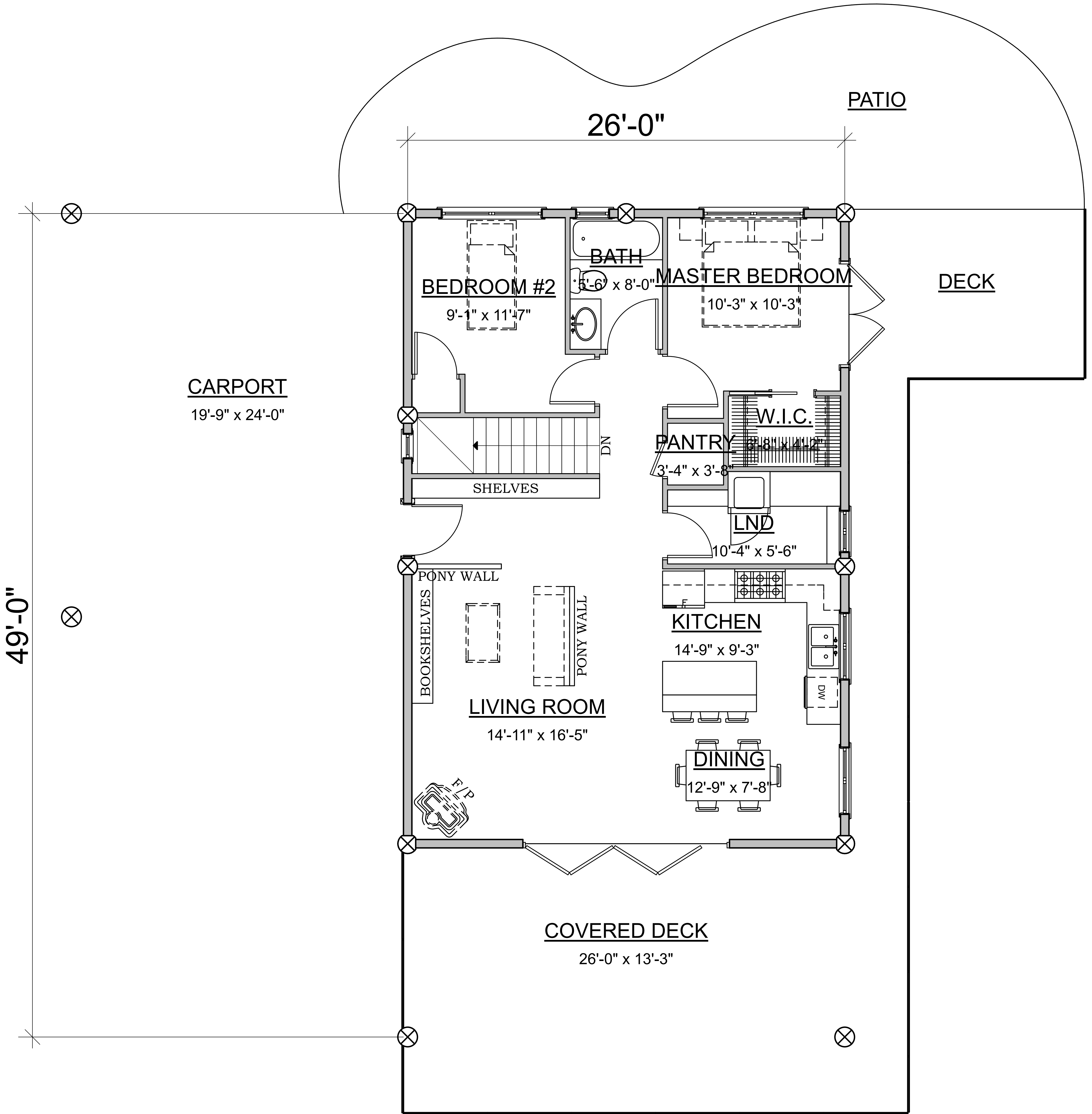
FIRST FLOOR PLAN AREA 965 sq ft
