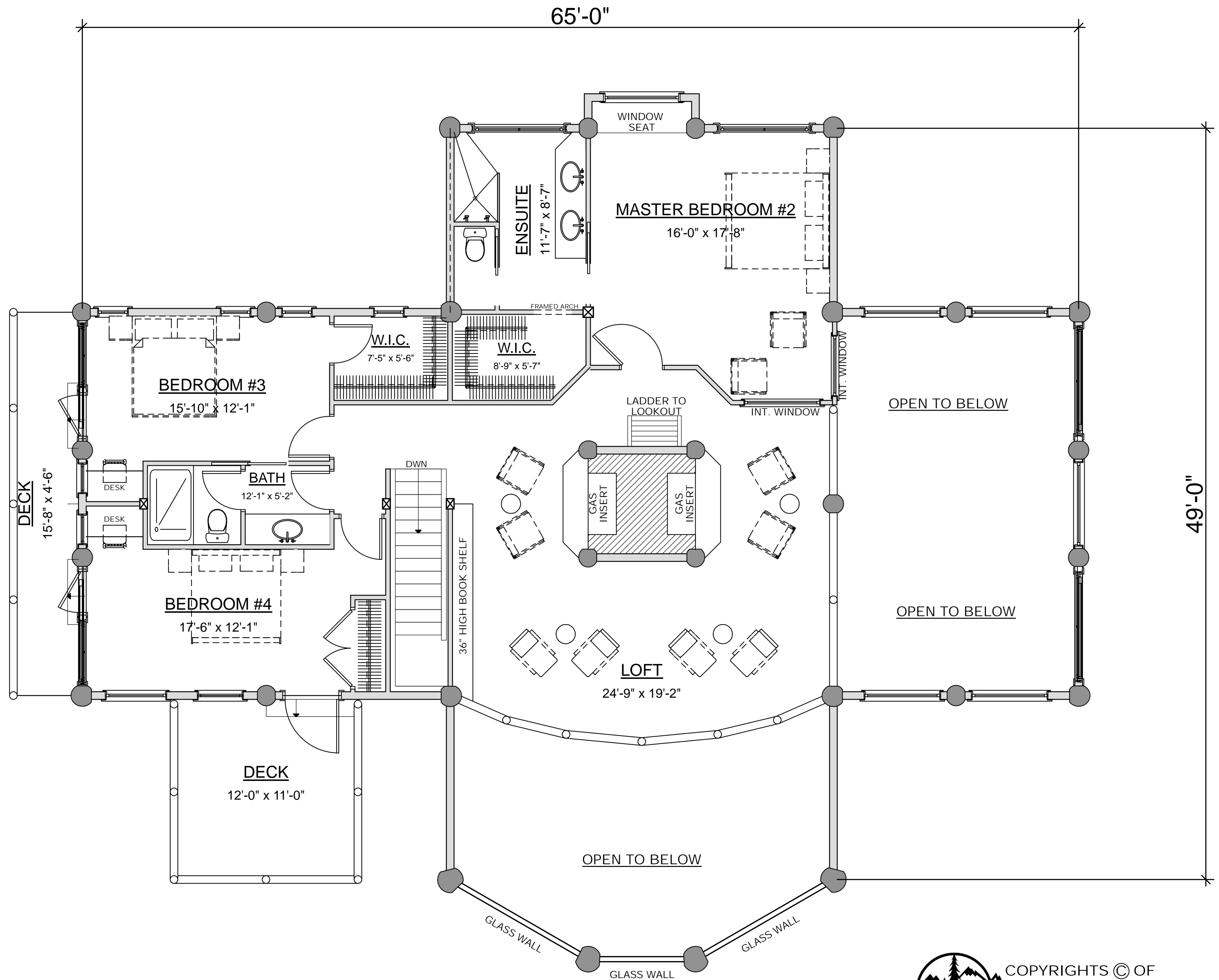
SECOND FLOOR PLAN AREA: 1,565 SQ. FT.
