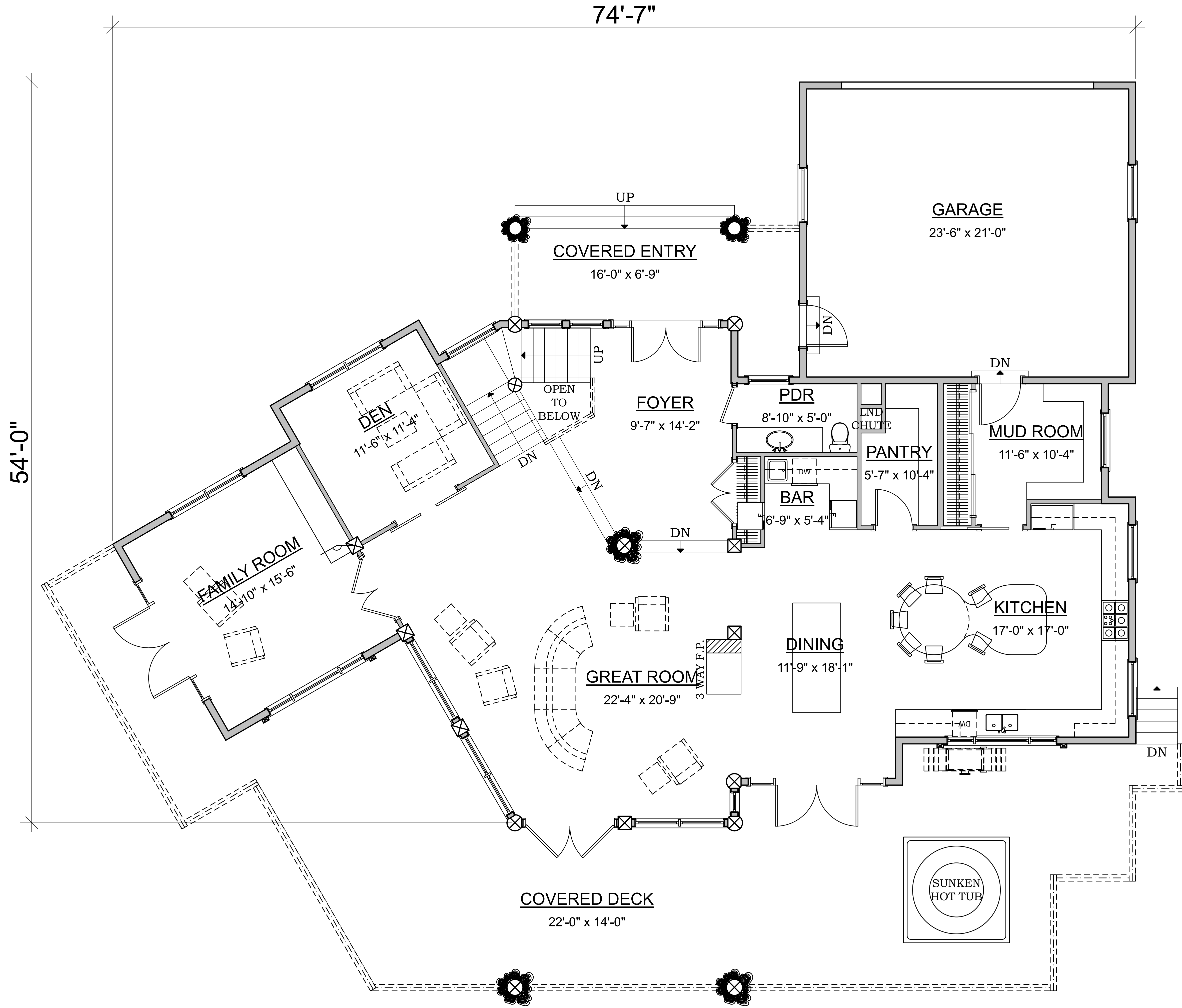
FIRST FLOOR PLAN AREA 1,985.93 sq ft
